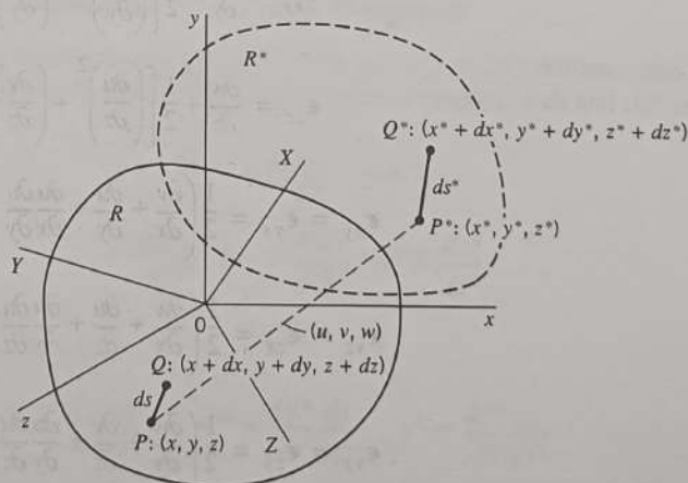
FIGURE 2.18 Line segment PQ in undeformed and deformed body.
