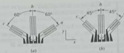
FIGURE 2.20 Rosette strain gages. (a) Delta rosette. (b) Rectangular rosette.
